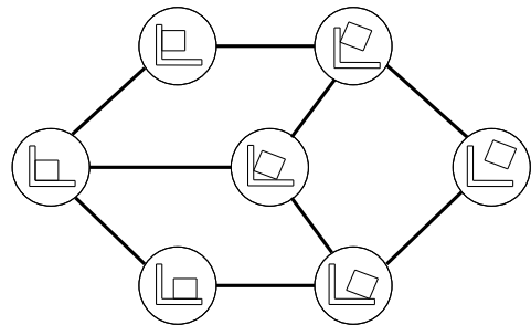
Fig. 3. A complete contact state graph shows all possible CFs (nodes) and transitions between neighboring CFs (arcs). While this figure shows a simplified example that only contains 7 CFs, a real contact state graph of two 3-dimensional polyhedral objects contains hundreds of CFs.
