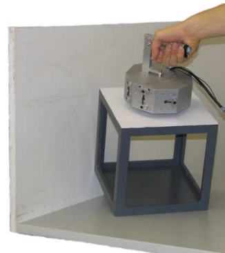
Fig. 1. In the experiment to validate the presented approach a cube is manipulated in contact with three perpendicular faces.
