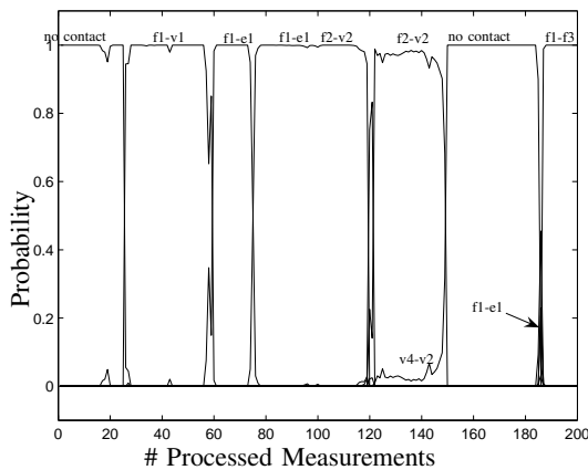
Fig. 7. The CF evolution of a human demonstration where a cube is manipulated in contact with two perpendicular faces. The evolution is shown by the probability on each of the CFs.
