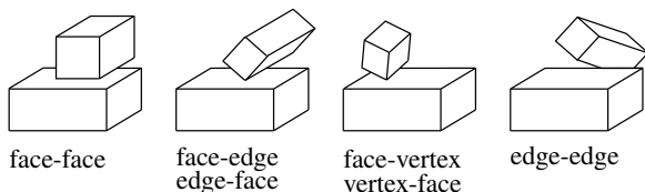
Fig. 2. The six possible non-degenerate principal contacts (PCs) between two polyhedral objects.
