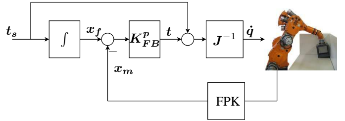
Fig. 5. The high speed Cartesian position feedback loop with velocity feedforward controls the joint velocities of the manipulator.
