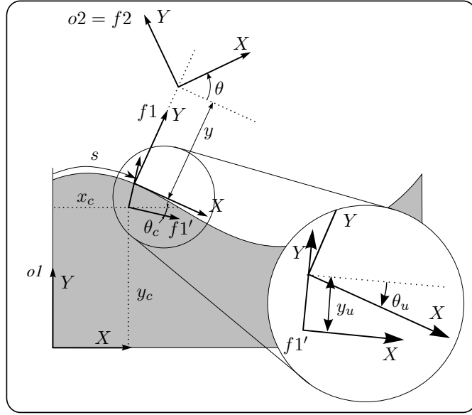
Figure 11: The feature coordinates and object and feature frames for the contour tracking example.
